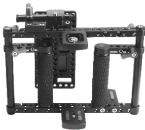
Folding state
