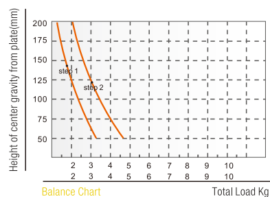
COUNTERBALANCE GRAPH
